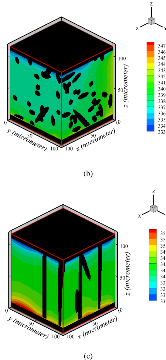
Fig2. The temperature distribution (in Kelvin) in the three layers of gas reconstructed: (a) \beta = 10000 , (b) \beta = 1 and (c) \beta = 0.01
